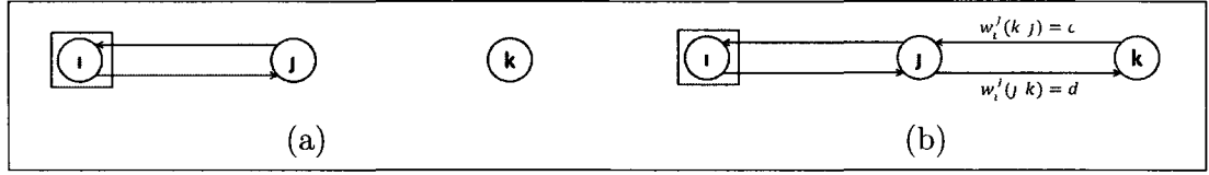
Figure 5.7 An illustration of the single-report-responsiveness property: there exists a subjective work graph G_i , e.g., the one shown in (a), such that a single positive report by j about k , as shown in (b), leads to S_{ik}^M(G_i, C_i) > S_0^M , and a single negative report by j about k leads to S_{ik}^M(G_i, C_i) < S_0^M .
