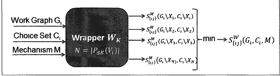
Figure 5.9 The K-Elimination-Wrapper
