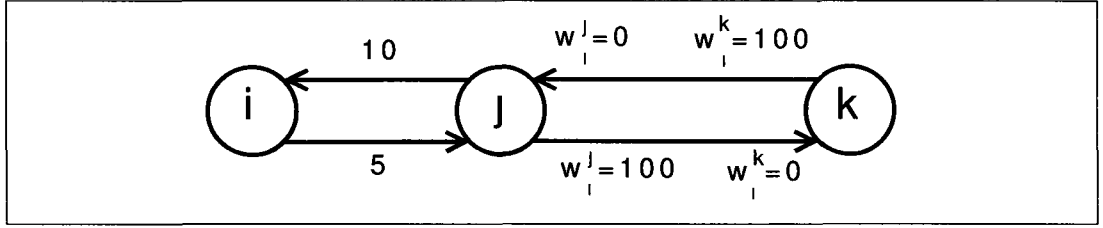
Figure 5.1 A subjective work graph from agent i 's perspective. Edges where i has direct information have only one weight. Other edges can have two weights, corresponding to the possibly conflicting reports of the two agents involved.
