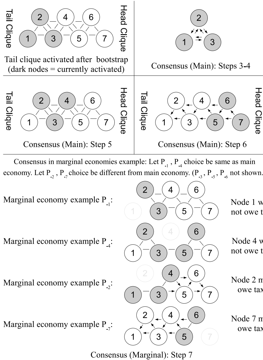
Figure 6.4: RaBC in action: consensus phases.
