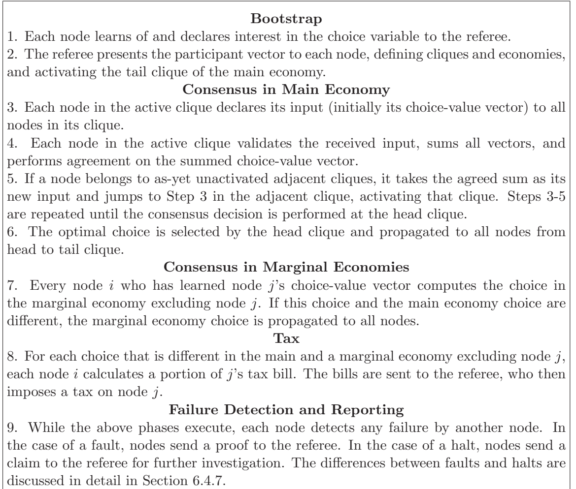
Figure 6.2: Overview of the suggested algorithm.
